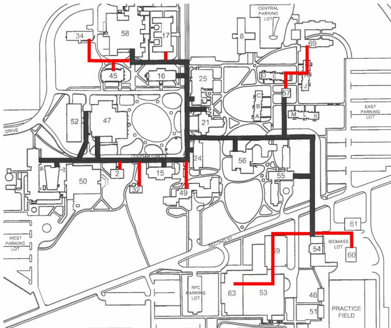
Figure 1. Distribution system tunnels and laterals routing
